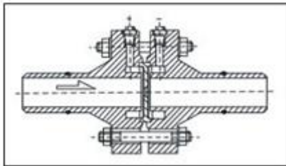
Tightening type eight-slot orifice plate PN \leq 10
