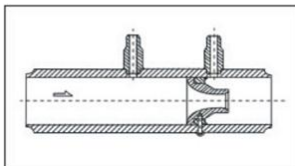
B: Long track nozzle
