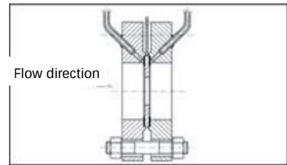
Standard orifice plate, bore-hole pressure tapping PN \leq 2.5
