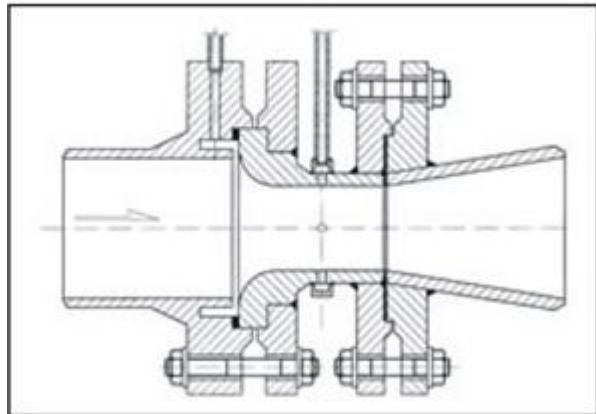
Venturi nozzle
