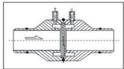
Welding type eight-slot orifice plate PN \leq 10 II
