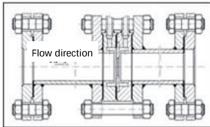
Standard orifice plate, annular chamber pressure tapping PN \leq 2.5
